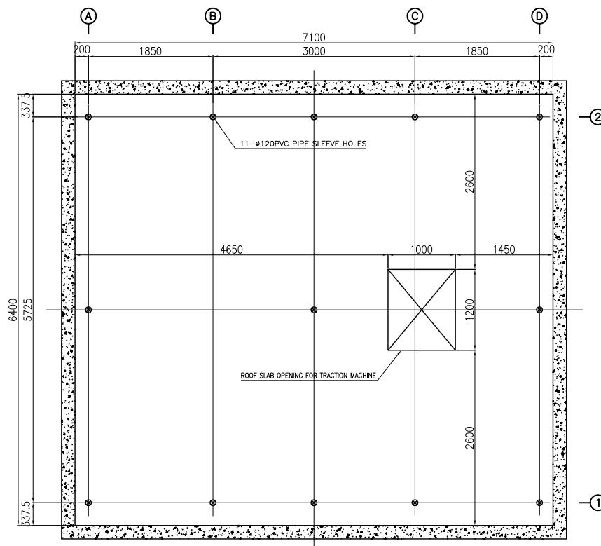
PLAN OF ROOF SLAB
