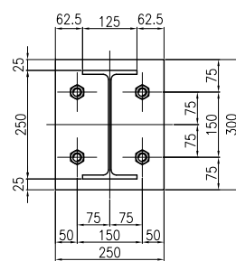
FOOT DETAIL PLAN
