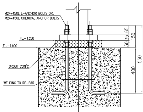
FOOT DETAIL
