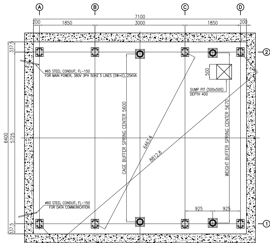
PLAN OF PIT
