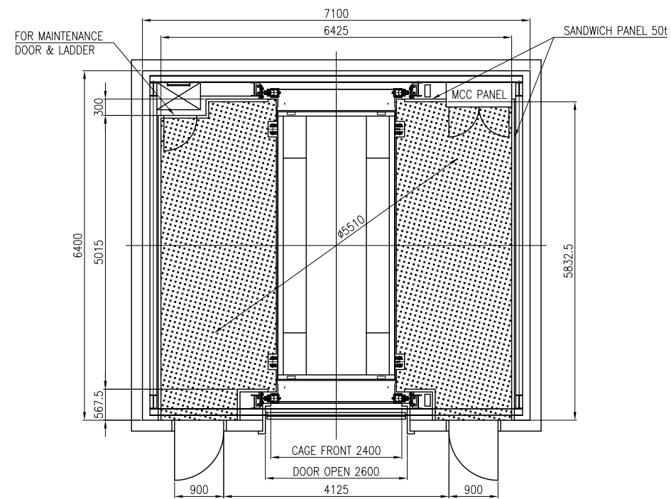
ENTRANCE PLATFORM PLAN
